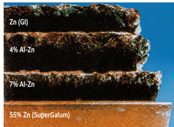
17-Year Exposure Test Results
